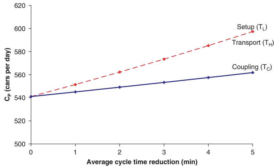
FIGURE 7 Pull-down capacity as function of cycle time reduction.
