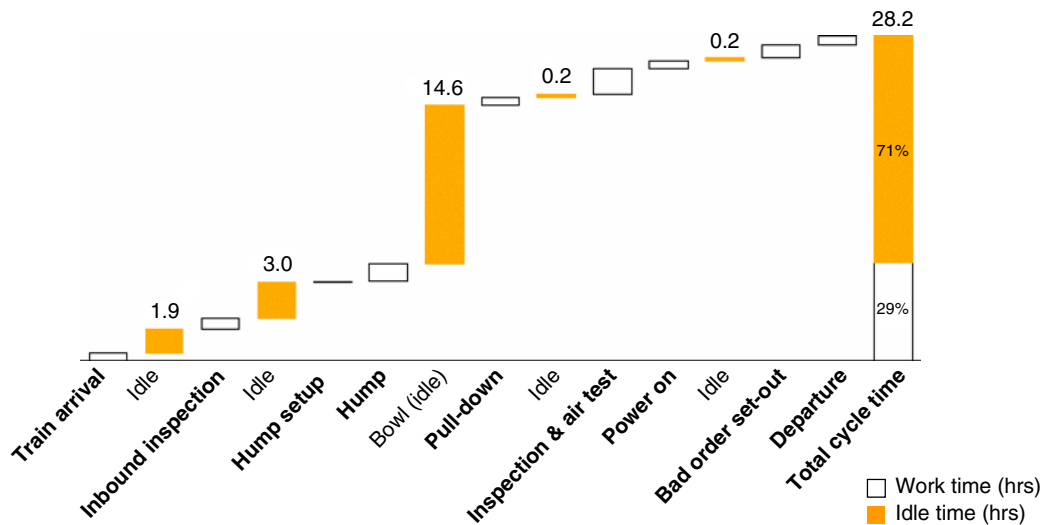
FIGURE 3 Average terminal process cycle time for major Class 1 railroad yard (5).
