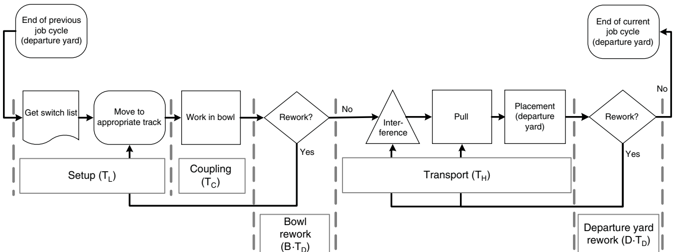
FIGURE 5 Pull-down process cycle time components.
