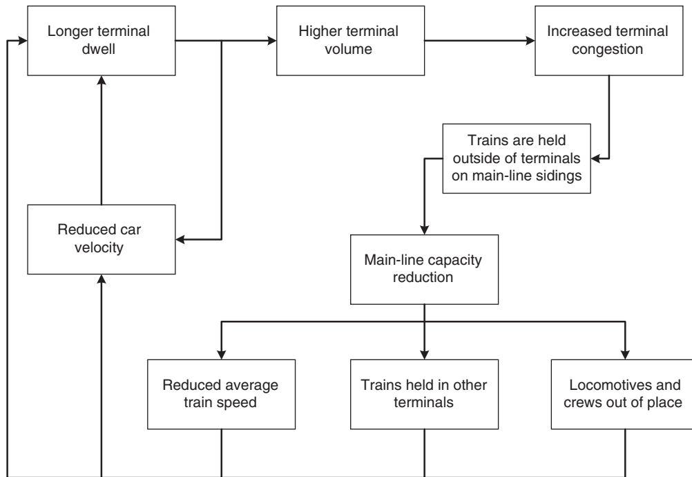
FIGURE 1 Railroad network efficiency cycle.
