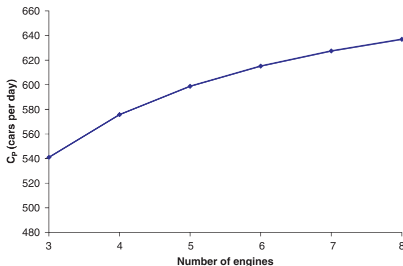
FIGURE 6 Pull-down capacity versus number of engines.
